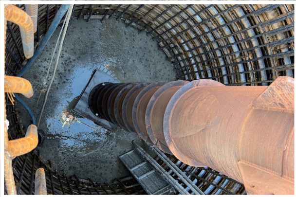
Foundation Installation
