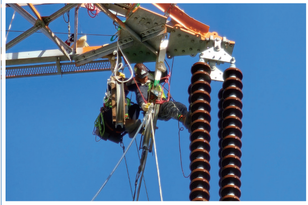
Insulator Installation
