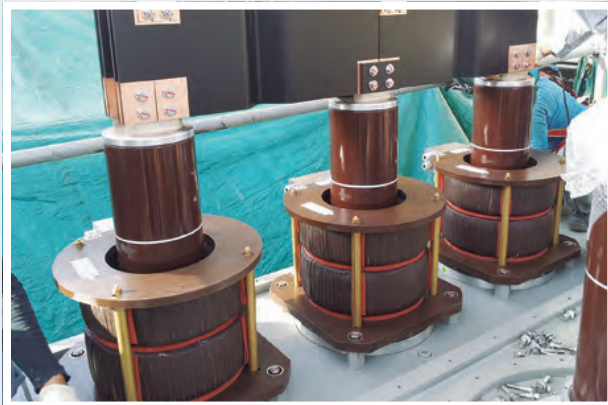
Assembling of generator CT
